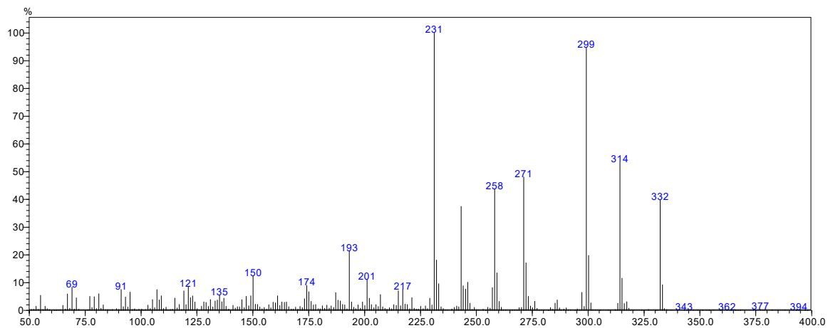
Figure 8. Electron-impact (70 eV) ionization mass spectrum of a standard of ( \pm )-9b-hydroxyhexahydrocannabinol analyzed by isothermal gas chromatography on a DB35ms column at 240 °C.
