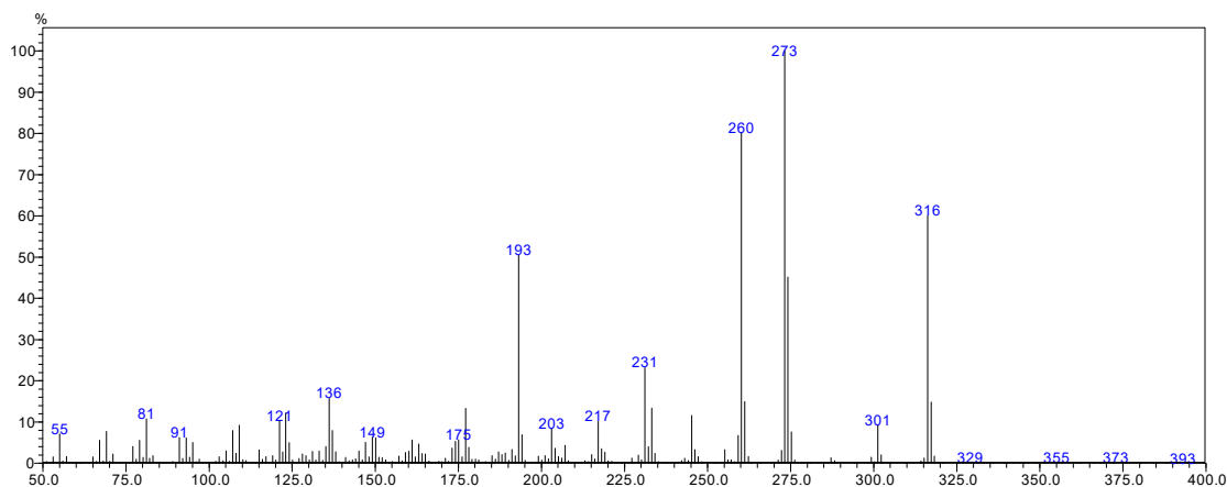
Figure 4. Electron-impact (-70 eV) mass spectrum of a reference standard of (6aR,9S,10aR)-HHC analyzed by isothermal gas chromatography on a DB35ms column at 240 °C.
