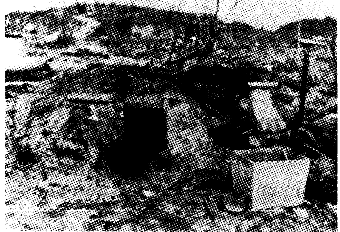
Fig. 1.5. Undamaged earth-covered family shelter in Nagasaki.
