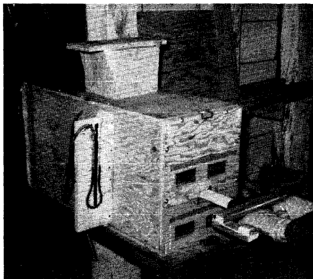
Fig. 5. Front End of the Durability Test Pump, showing the lower fixed part (below piston rod) and the upper removable part, that is held by 6 screws with flat washers. Felt weather-stripping makes the removable part airtight.
