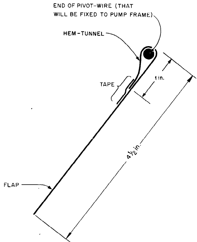
Fig. 7. End view.
