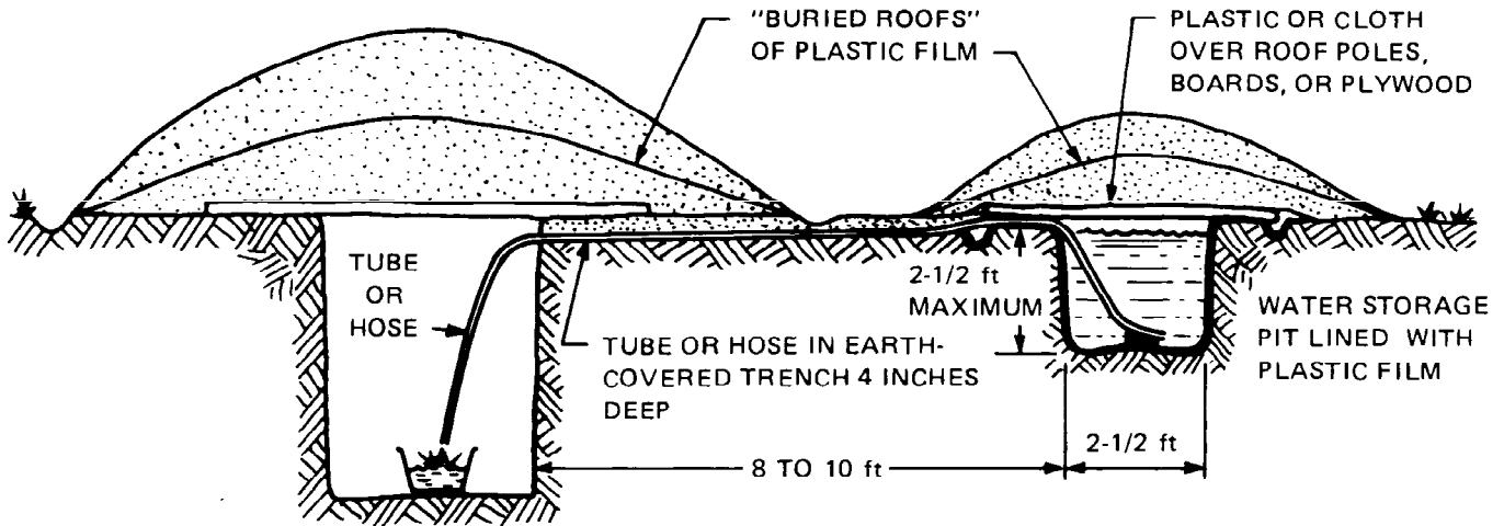
Fig. 8.7. Water siphoned into a belowground shelter.
