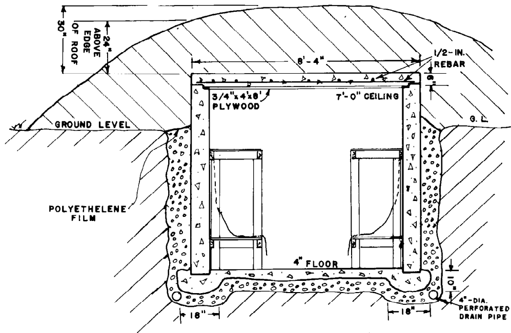
SECTION B-B'
