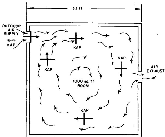
Fig. 16. The use of air-distribution KAPs.
