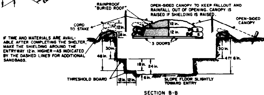
Fig. A.1. Door-Covered Trench Shelter.
