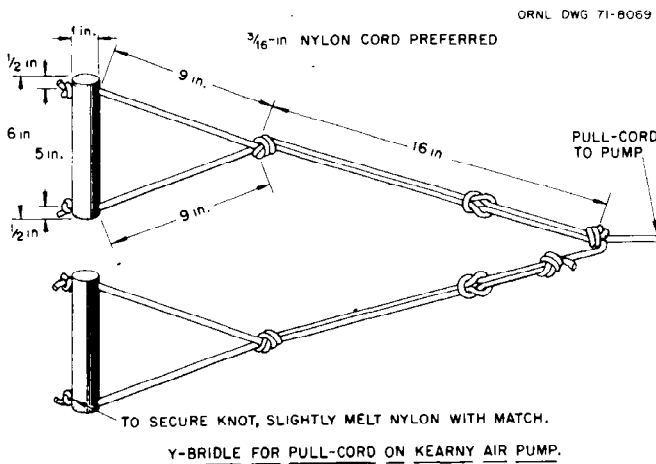
Fig. 23. Y-bridle for pull-cord on KAP.
