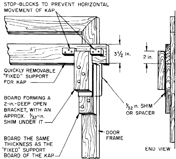
Fig. 19. Quick-removal bracket for KAP.
