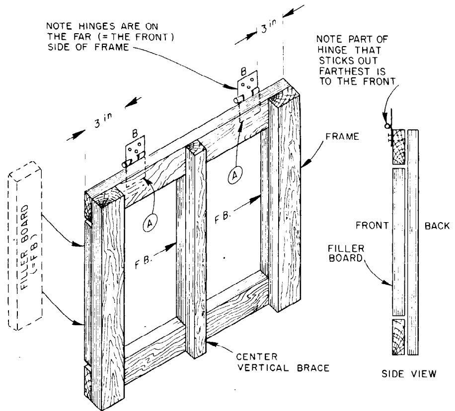
Fig. 4. Completing the frame.
