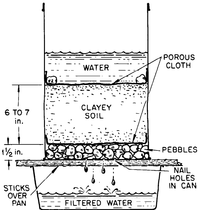
Fig. 8.11. Expedient filter to remove radioactivity from water.
