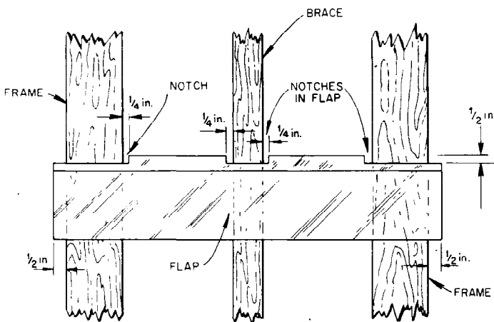
Fig. 6. Sizes of notches in flaps.
