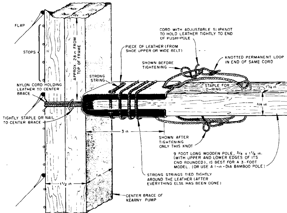
Fig. 26. Push-pole flexible connection.
