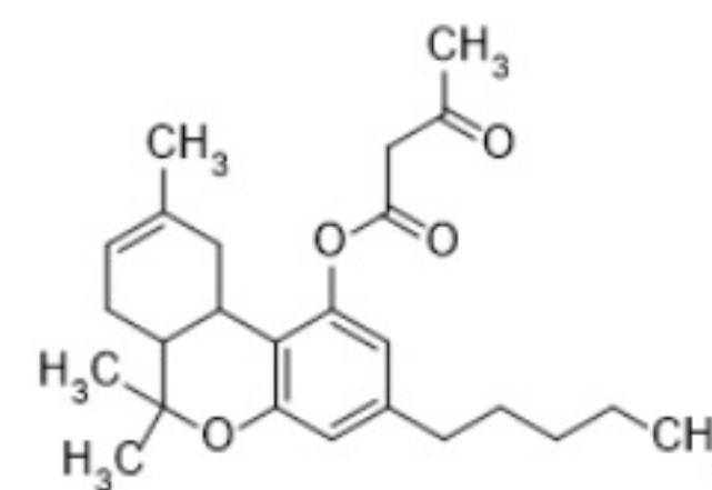
Delta-8 Tetrahydrocannabinyl Acetoacetate (D8 THC Acetoacetate)
