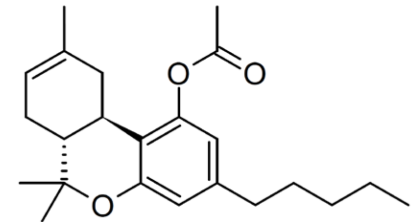
Delta-8 THC-O Molecule
