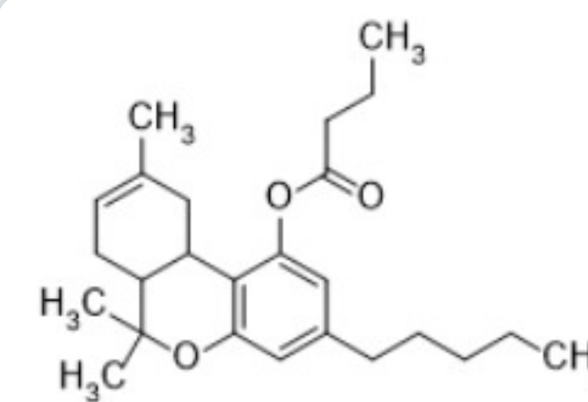
Delta-8 Tetrahydrocannabinyl Butyrate (D8 THC Butyrate)
