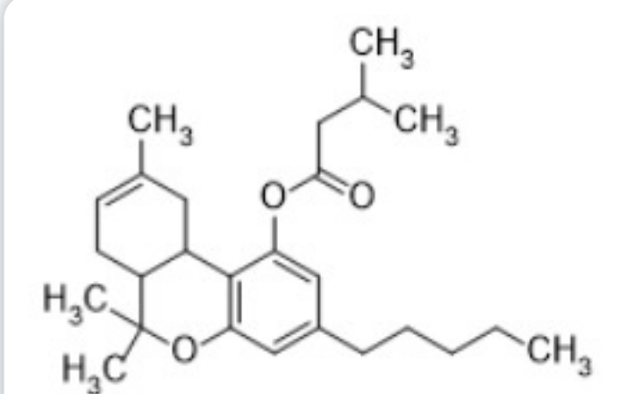
Delta-8 Tetrahydrocannabinyl Isovalerate (D8 THC Isovalerate)
