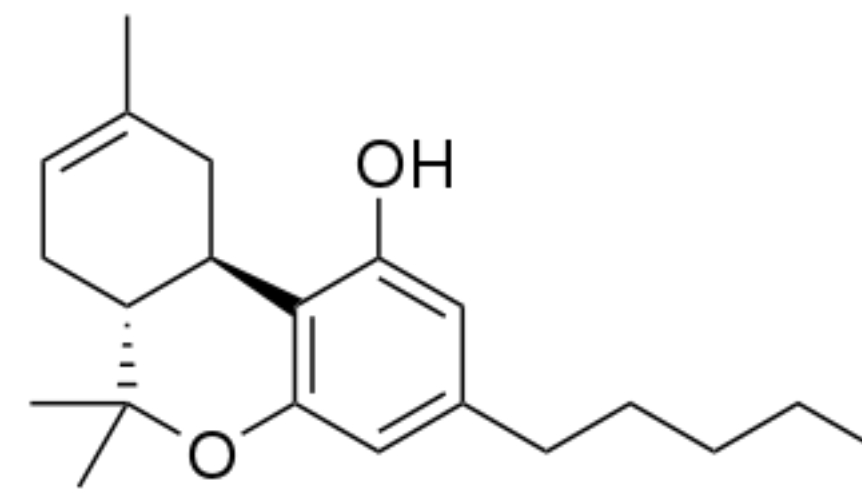
Standard Delta-8 THC Molecule
