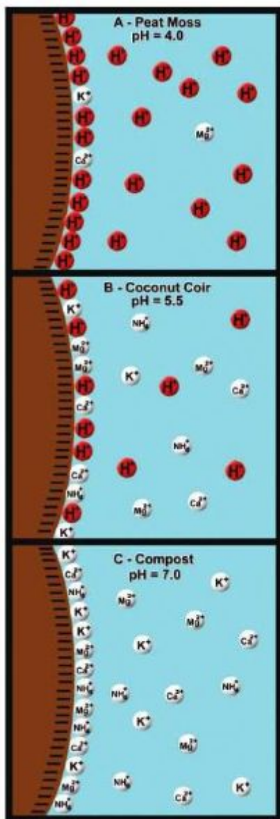
Figure 2. Box A represents unlimed peat moss with a pH of 4.0. Here, most of the negative charges on the surface of the peat are occupied by acidic \text{H}^+ ions, with a few sites occupied by nutrient ions ( \text{Ca}^{2+} , \text{Mg}^{2+} , \text{K}^+ or \text{NH}_4^+ ). There is also a large number of acidic \text{H}^+ ions in the solution surrounding the substrate particles. Most of this acid needs to be neutralized by limestone in order to make the peat suitable for cannabis production.
