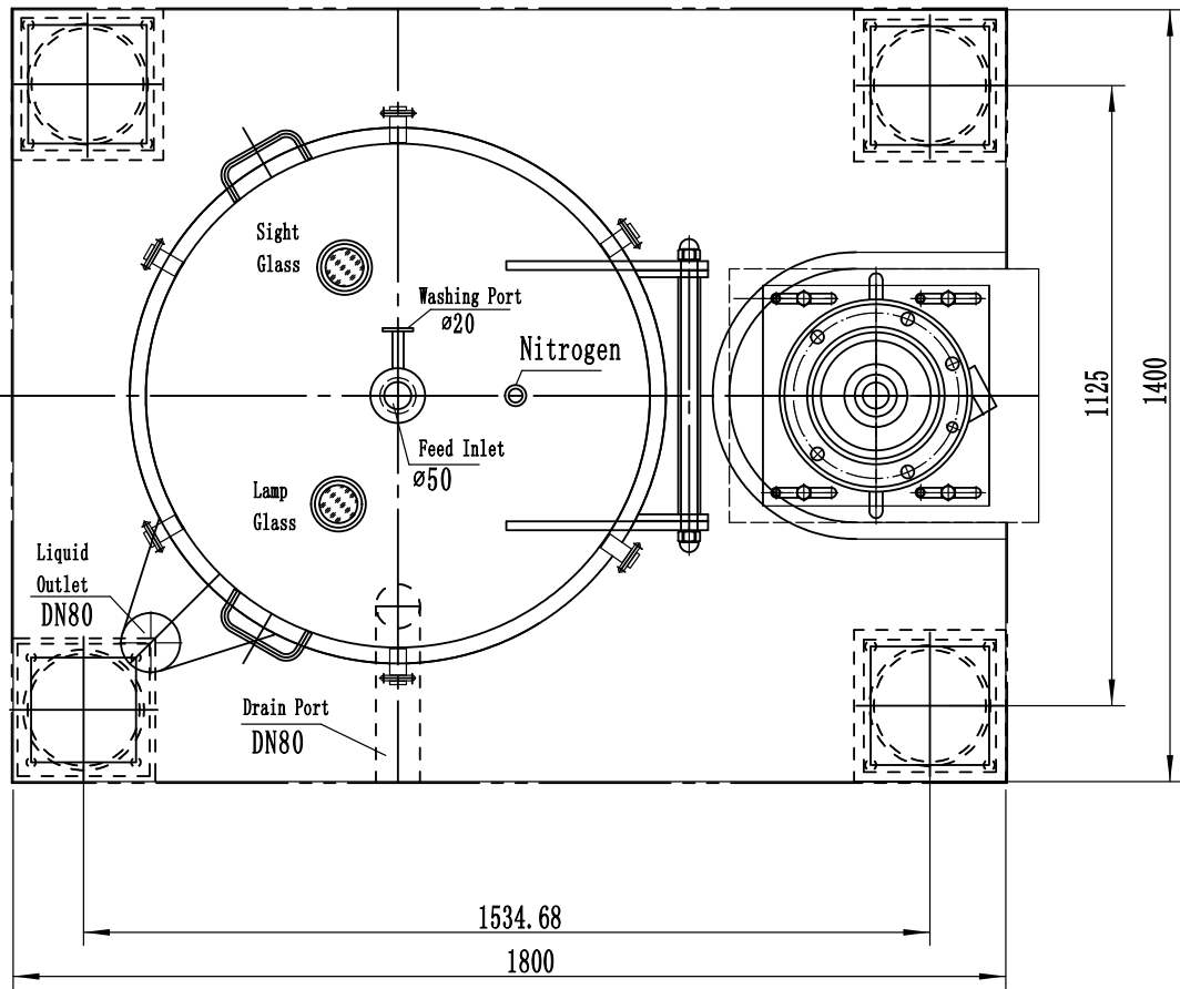
PS600 Soak and Filter Centrifuge
